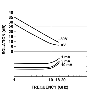
Figure 1. Typical Isolation and Insertion Loss, HPND-4028.
